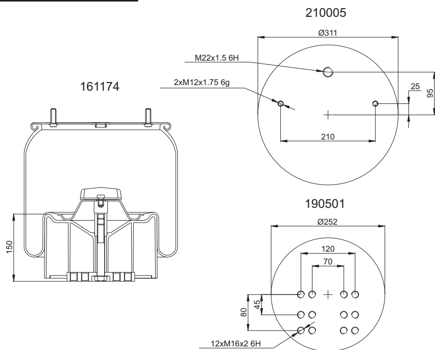
(Composite Piston)
