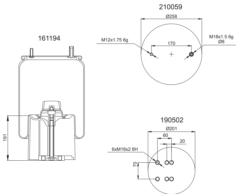
(Composite Piston)
