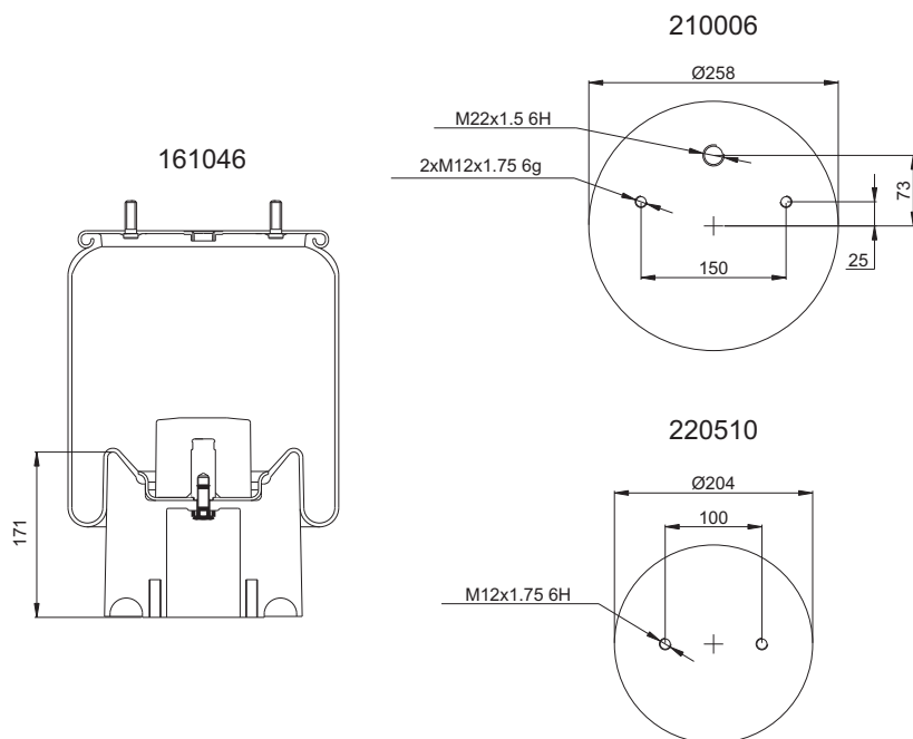
(Composite Piston)
