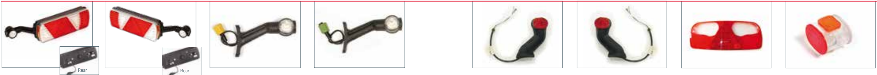
Left-hand rear light LED version with white light cover panel and plug including tracking light Item no. 6606445 Right-hand rear light LED version with white light cover panel and plug including tracking light Item no. 6606444 Left-hand tracking light LED version with cable for ID 6606445 Item no. 6503124 Right-hand tracking light LED version with cable for ID 6606444 Item no. 6503123 Left-hand tracking light Red/white glass for ID 6603167 Item no. 6000010 Right-hand tracking light Red/white glass for ID 6603166 Item no. 6000011 Left and right-hand lighting cover panel Light cover for left and right use f or ID 6603167, 6603166 Item no. 6500139 Left and right-hand lighting cover panel Can be used for tracking light for ID 6603166, 6603167, 6000010, 6000011 Item no. 6500140
