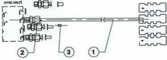
FOOT BRAKE VALVE
