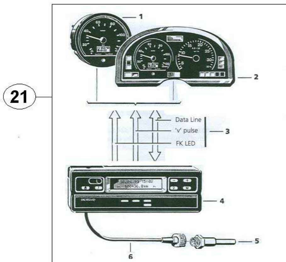
Fig. 1-4: System variant; MTCO - K-Line and Electronic Speedometer/ Cluster
