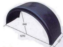
TD07-63-009 (OLD:TD-50-209) UNIVERSAL FENDER SKIRT 1270X520
