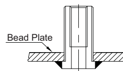
Combination stud/air inlet (Combo Stud)
