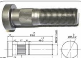
AA0015 SAF Type Single To replace OE 1303107412
