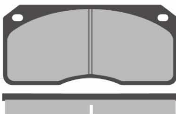
AD8240 4 Identical Pads 177 x 77 x 22mm WVA29302
