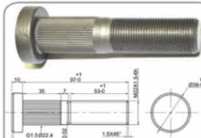
AA0017 BPW Type To replace OE 0329633120
