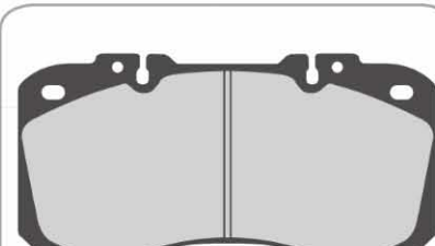
AD8050 4 Identical Pads 175 x 86 x 22mm WVA29159
