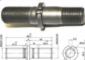
AA0012 BPW Type To replace OE 0329623150
