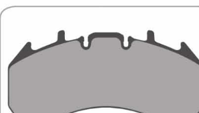
AD8140 4 Identical Pads 165 x 66 x 17mm WVA29121
