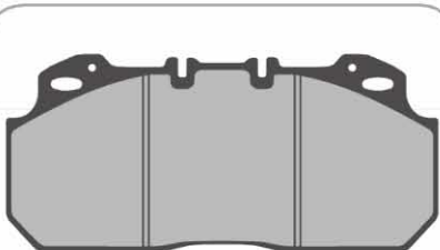
AD8040 4 Identical Pads c/w Fitting Ring 250 x 114 x 28mm WVA29090
