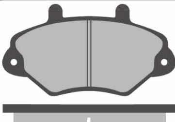
AD8270 4 Identical Pads 138.8 x 72 x 18mm WVA21469
