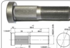
AA0024 BPW Type, To replace OE 0329633141
