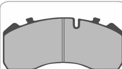
AD8020 4 Identical Pads 211 x 92.5 x 30mm WVA29093/095
