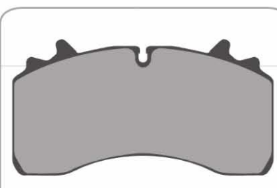
AD8110 4 Identical Pads 210 x 110 x 30mm WVA29162
