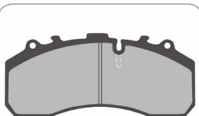
AD8200-AD620 4 Identical Pads 248 x 108 x 30mm WVA29087 (988) Hi-Grade
