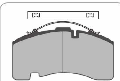
AD8080 4 Identical Pads 210 x 108 x 29mm WVA29171
