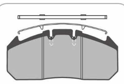
AD8090 4 Identical Pads 250 x 118 x 30mm WVA29131
