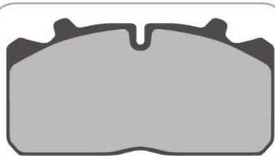
AD8000 4 Identical Pads 176 x 86 x 26mm WVA29088
