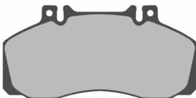
AD8320 4 Identical Pads 175 x 86 x 22mm WVA29065
