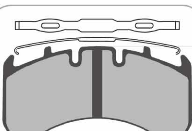
AD8100 4 Identical Pads 210 x 100 x 30mm WVA29169
