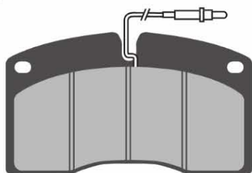
AD8260 2 Plain Pads, 2 pads c/w Wear Indicators 169.8 x 98 x 19mm WVA29072
