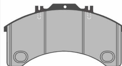
AD8310 4 Identical Pads 241 x 125 x 25mm WVA29011
