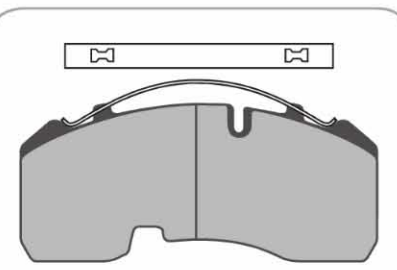
AD8060 4 Identical Pads 210 x 92 x 29mm WVA29165
