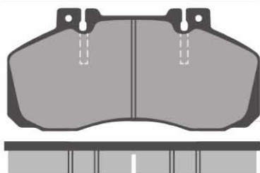
AD8230 4 Identical Pads 173 x 83 x 21.5mm WVA20835/29835
