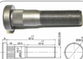
AA0014 Meritor 9000 Single To replace OE 21220969
