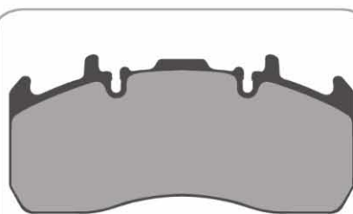
AD8190 4 Identical Pads 216 x 97 x 29mm WVA29173
