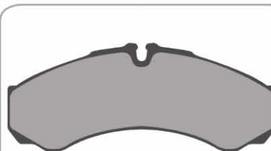
AD8140 4 Identical Pads 165 x 66 x 17mm WVA29121
