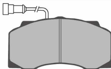
AD8010 2 Plain Pads, 2 pads c/w Wear Indicators 205 x 106 x 27mm WVA29077/092
