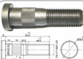
AA0004 LH 7/8" BSF Twin To replace OE 21018491
