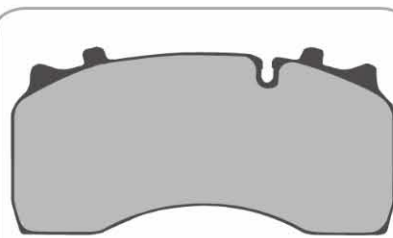
AD8210 4 Identical Pads 204.6 x 99.6 x 30mm WVA29119/29141
