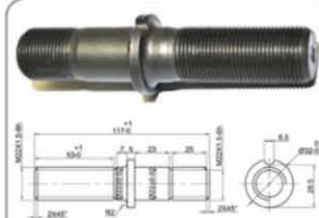
AA0011 SAF Type To replace OE 1303104010
