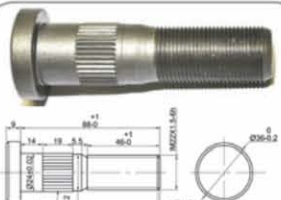
AA0005 RH M22x1.5mm ISO Single To replace OE 21022167
