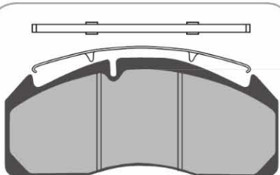
AD8030 4 Identical Pads 250 x 111 x 30mm WVA29125
