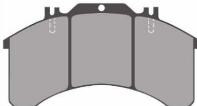
AD8300 4 Identical Pads 206 x 107 x 25mm WVA29032
