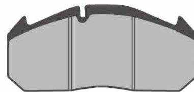
AD8280 4 Identical Pads 250 x 118 x 28mm WVA29030/29113
