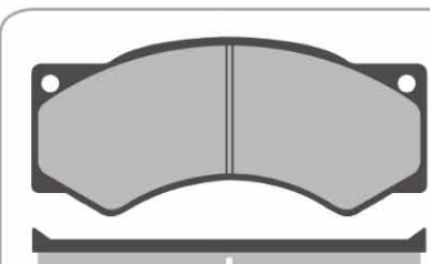
AD8220 4 Identical Pads 191 x 87 x 23mm WVA29017
