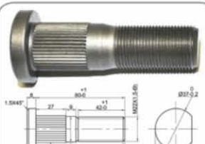
AA0016 SMB Type Single To replace OE CF101634
