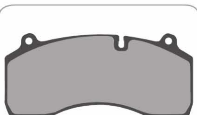
AD8180 4 Identical Pads 211 x 94 x 30mm WVA29147/29181
