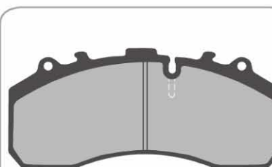
AD8200 4 Identical Pads 248 x 108 x 30mm WVA29087 (988)
