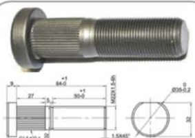
AA0018 SAF 9000 Single Steel To replace OE 1303107410
